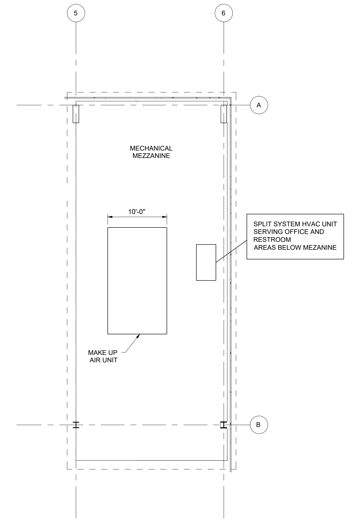
LEVEL 2 MECHANICAL DIAGRAM 1/8" = 1'-0"
