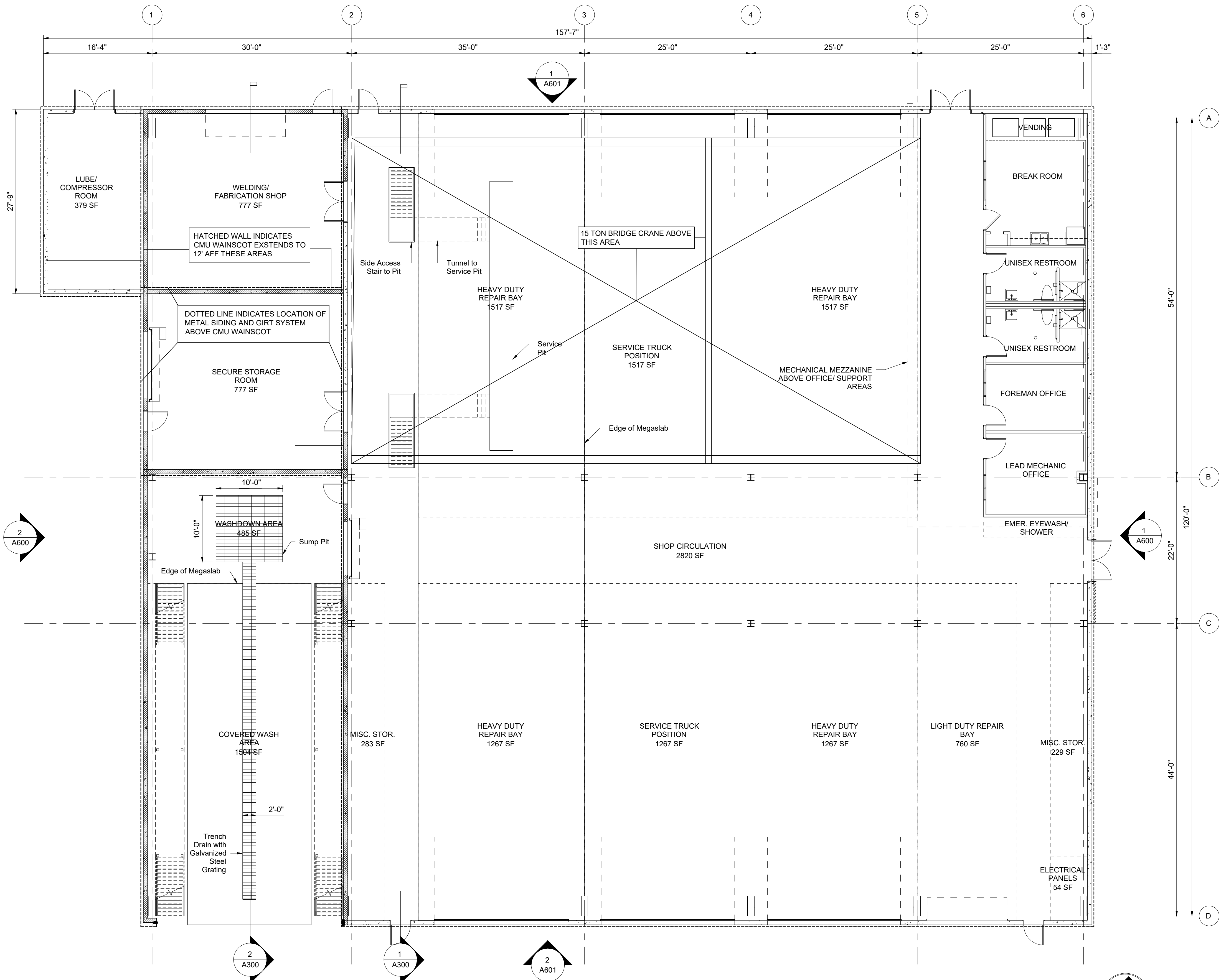
NORTH FLOOR PLAN 1/8" = 1'-0"
