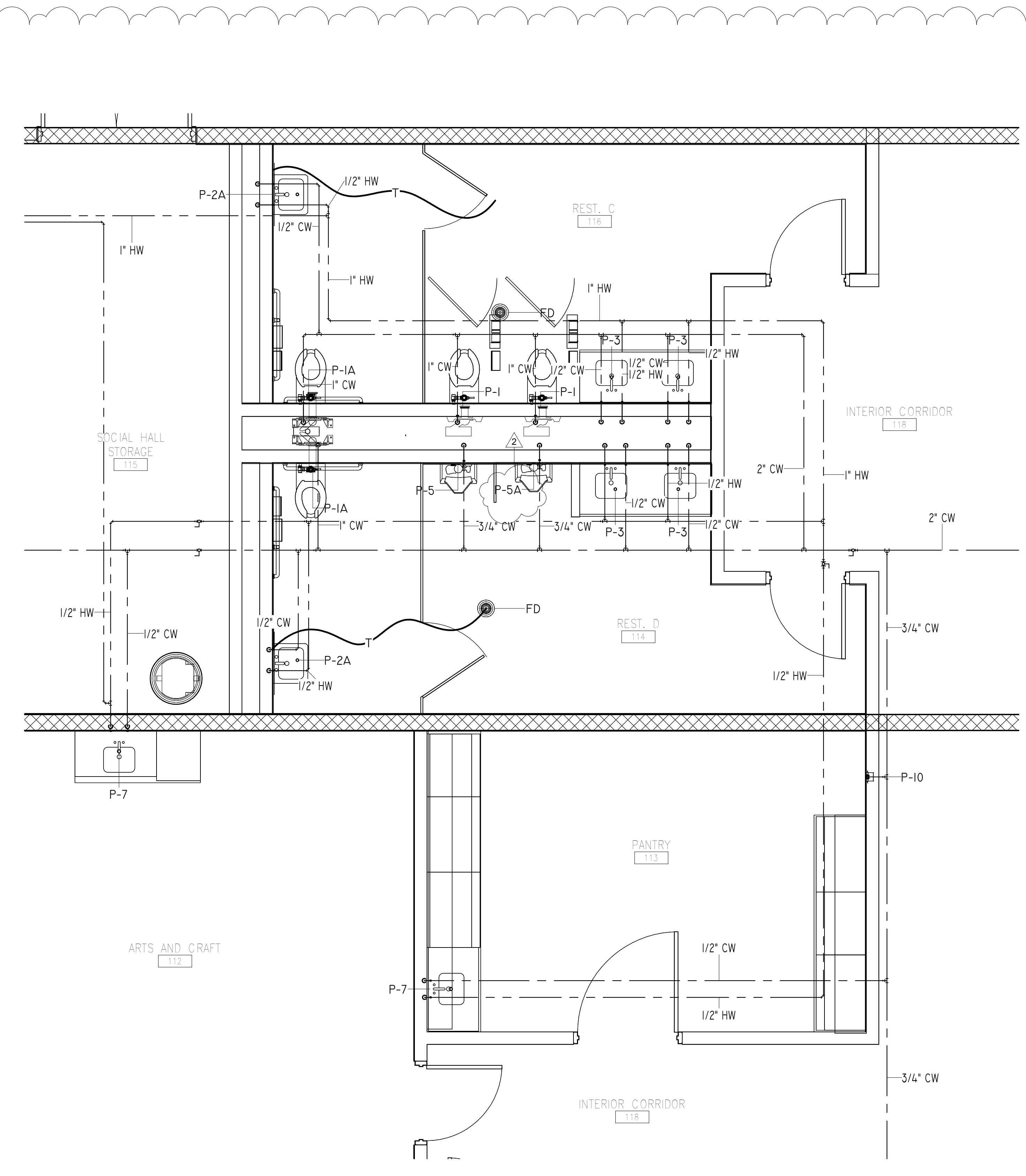
DOMESTIC PIPING NEW WORK ENLARGED PLAN - RESTROOM C/D SCALE: 3/8" = 1' - 0"
