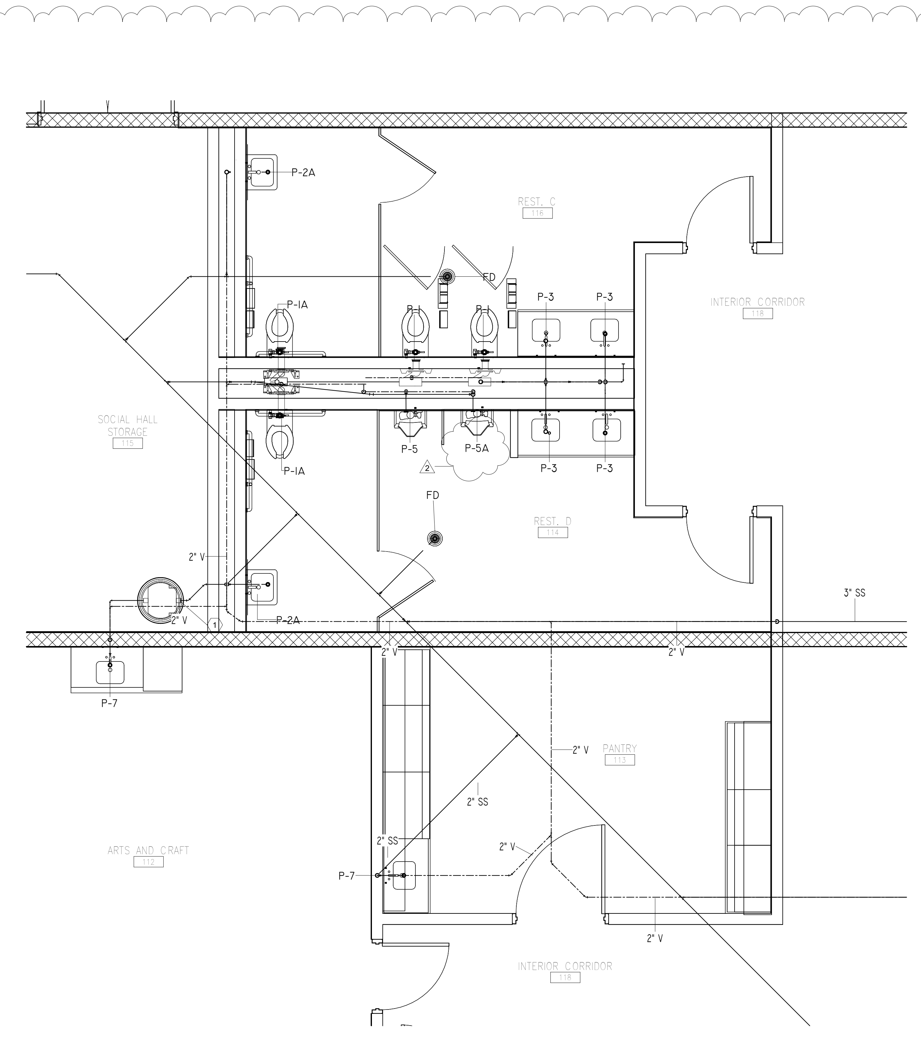
SANITARY PIPING NEW WORK ENLARGED PLAN - RESTROOM C/D SCALE: 3/8" = 1' - 0"
