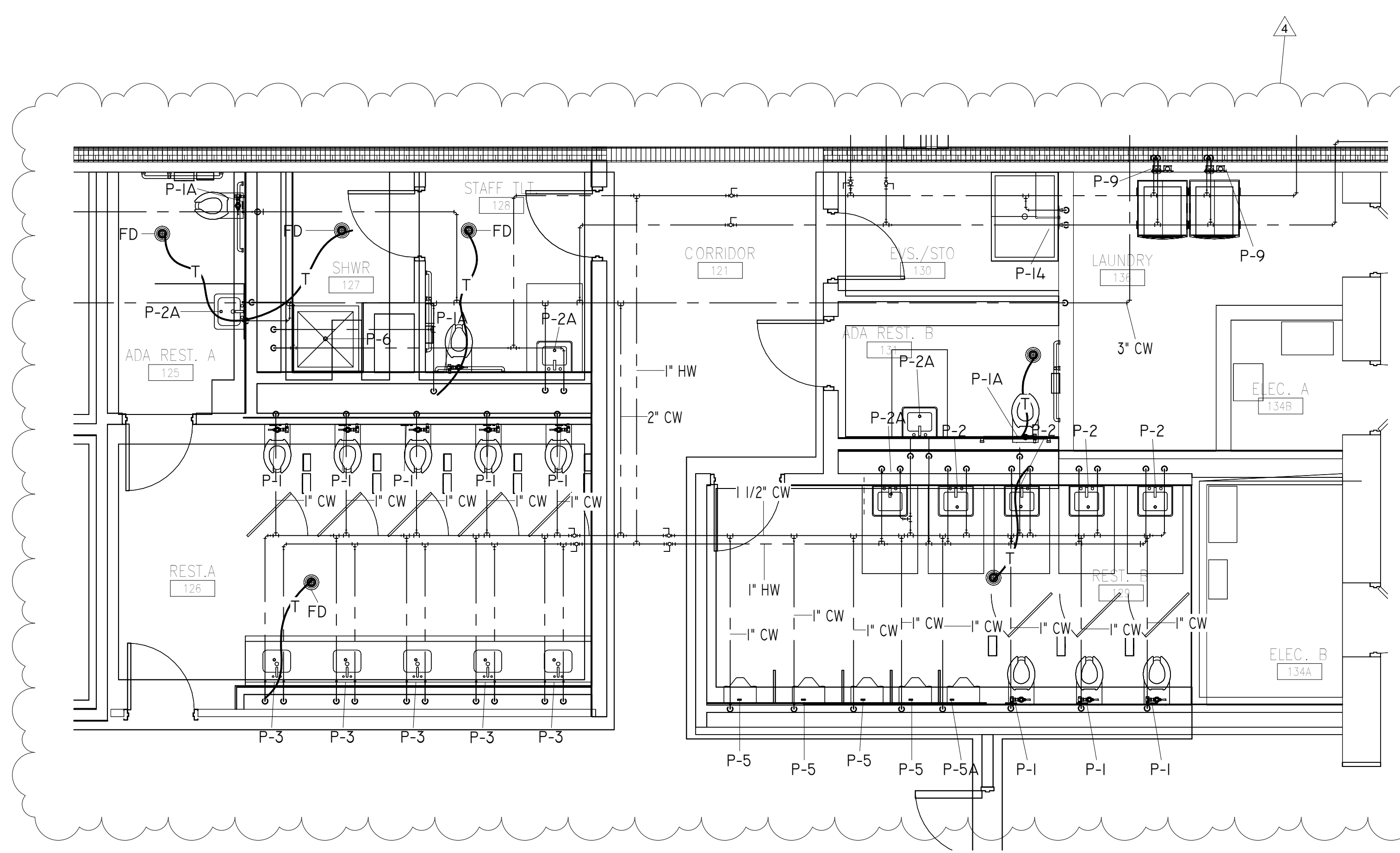
DOMESTIC PIPING NEW WORK ENLARGED PLAN - RESTROOM A/B
