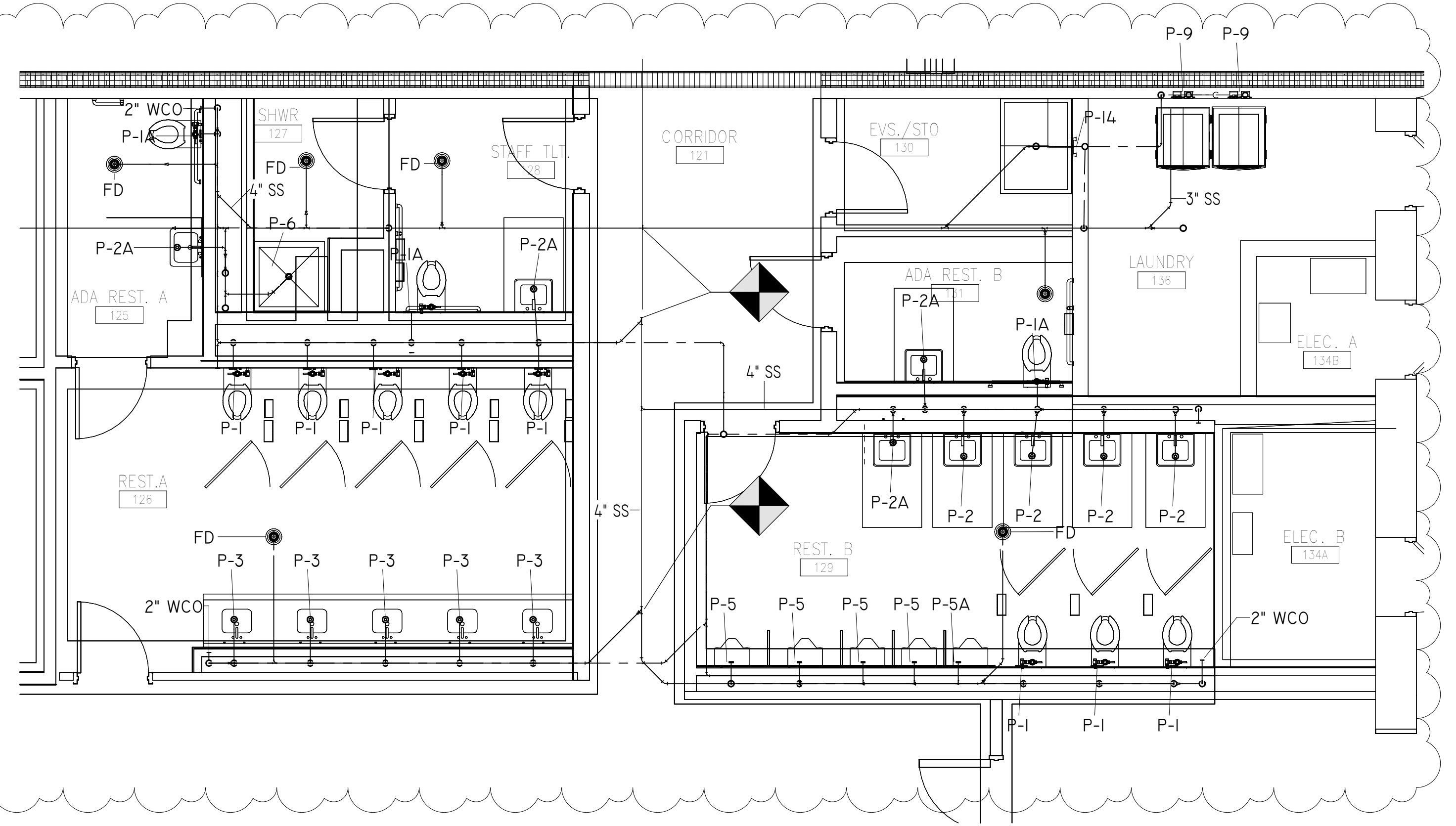
SANITARY PIPING NEW WORK ENLARGED PLAN - RESTROOM A/B
