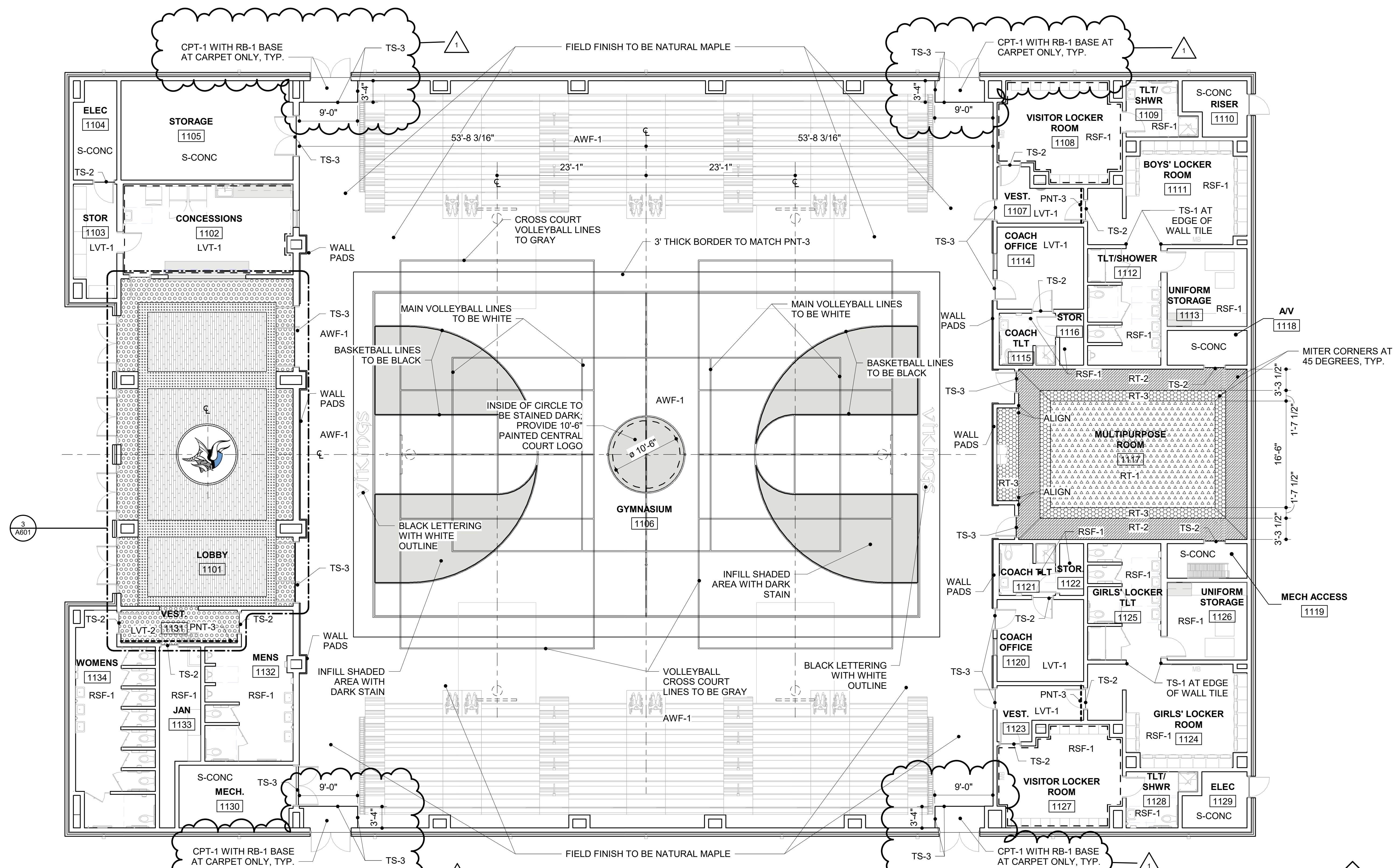
1 FLOOR PATTERN AND FINISH PLAN 1/8" = 1'-0"
