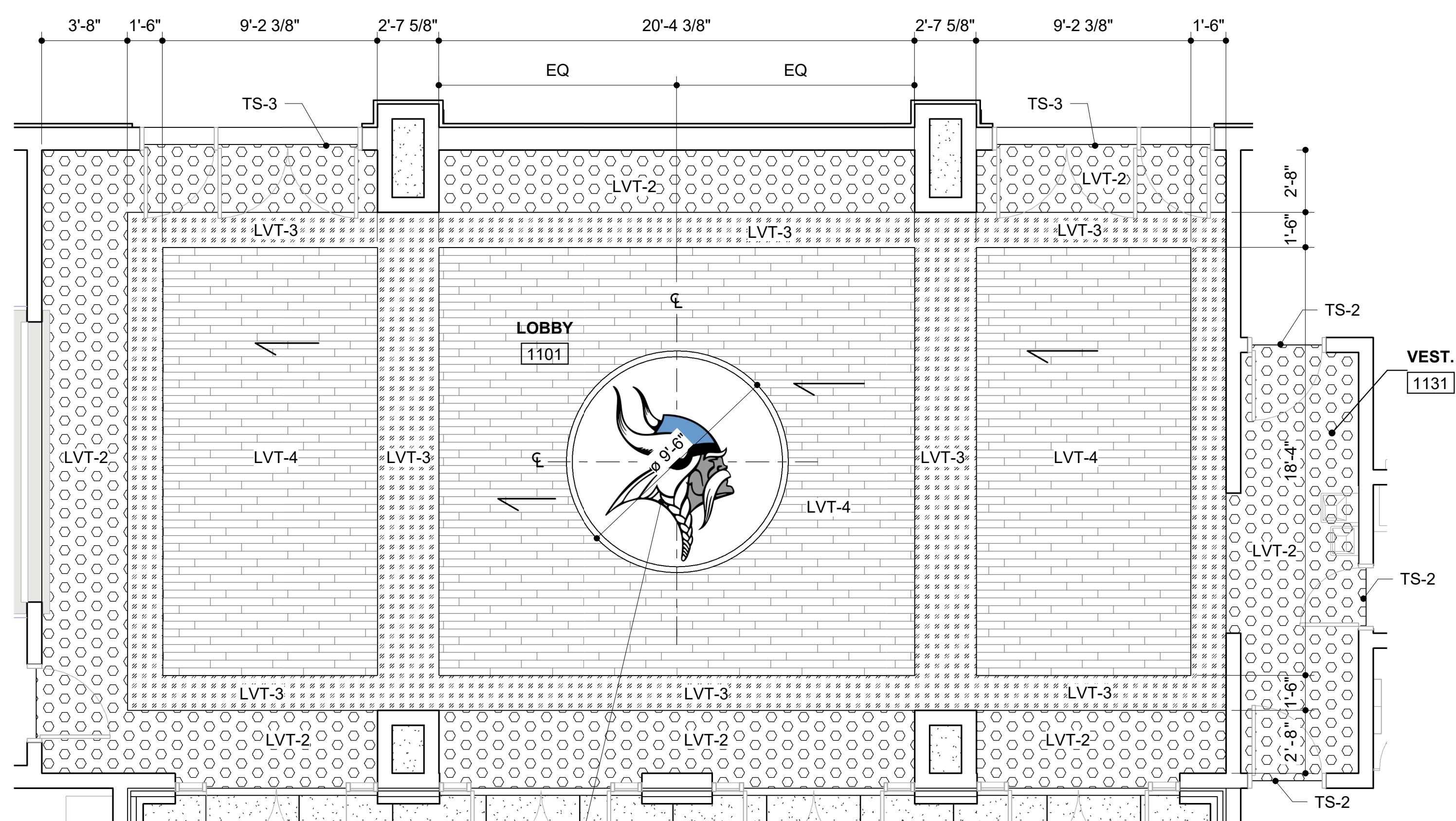
3 ENLARGED LOBBY FLOOR PATTERN PLAN 1/4" = 1'-0"
