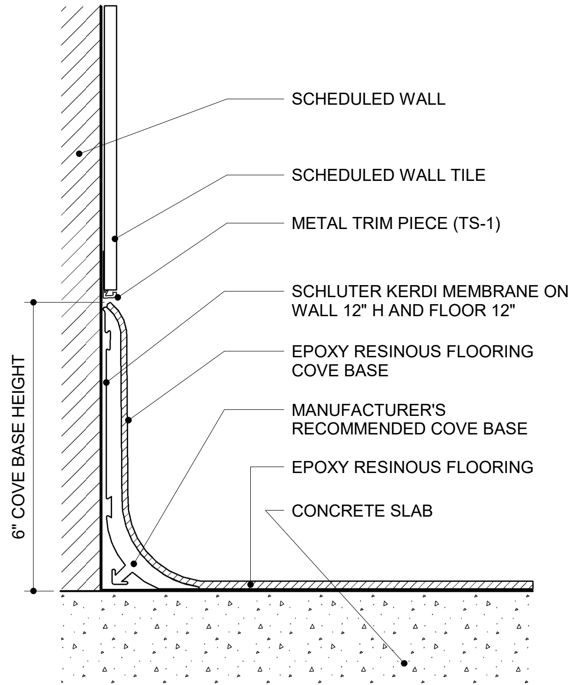
② RESINOUS FLOORING BASE DETAIL 6" = 1'-0"
